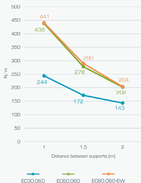
Safe working loads 60mm width basket trays
